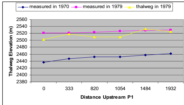
Figure 6 Calibration of the thalweg of Legagdadi reservoir
