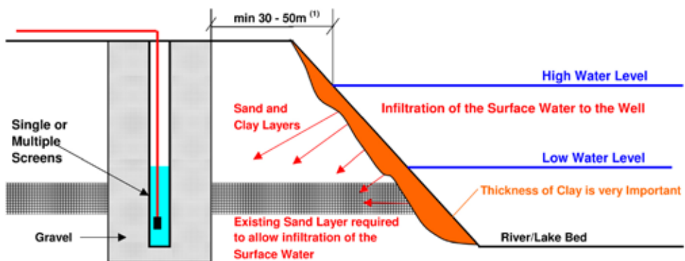
Figure 3: Typical design of RBI
