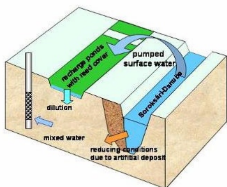
Figure 4: RBI with recharge ponds
