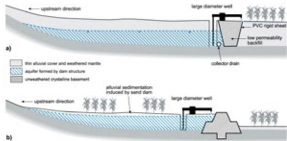
Figure 1: Typical design of subsurface dam (Source: GWMATE)
