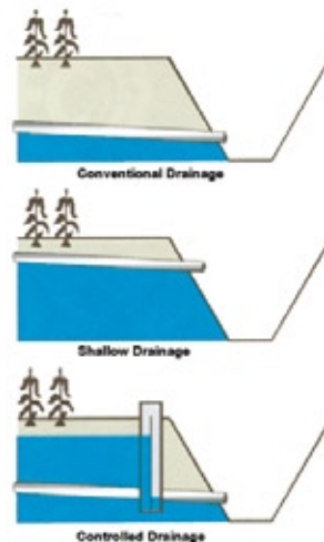
Figure 1: Various piped drainage systems
