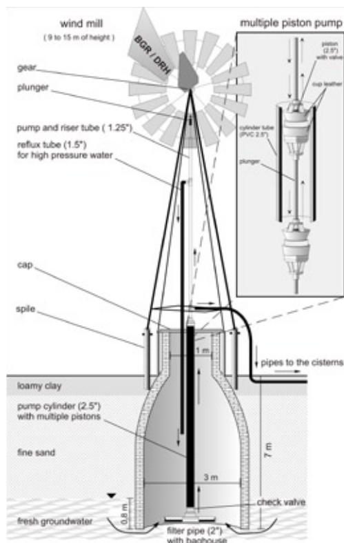
Figure 4: Schematic overview of windmill
