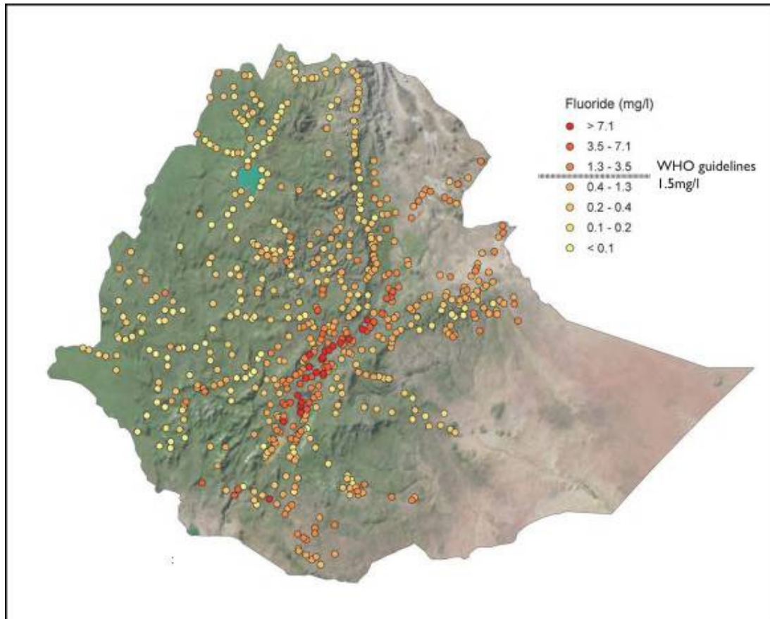
Figure 7: Occurrence of fluoride in groundwater
